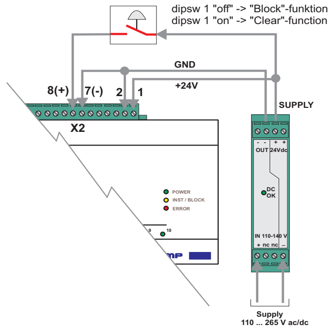
Figure 7.2-1. Binary input
