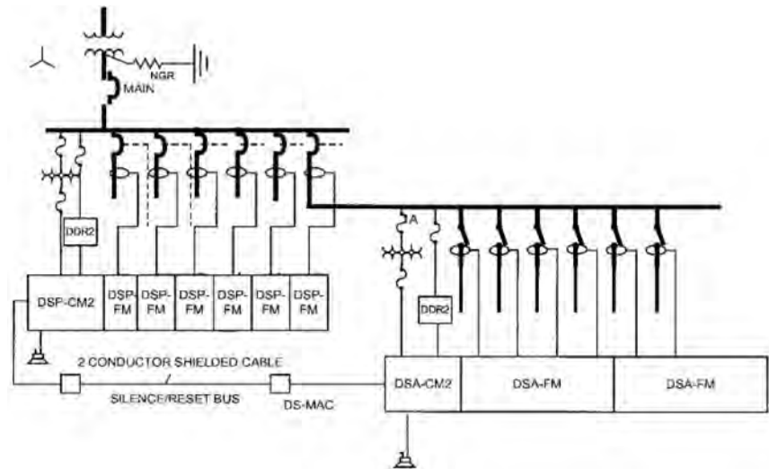
FIGURE 10.3.3 (A): TWO-LEVEL GROUND FAULT SYSTEM WITH DSP ON MAINS AND DSA ON FEEDERS
