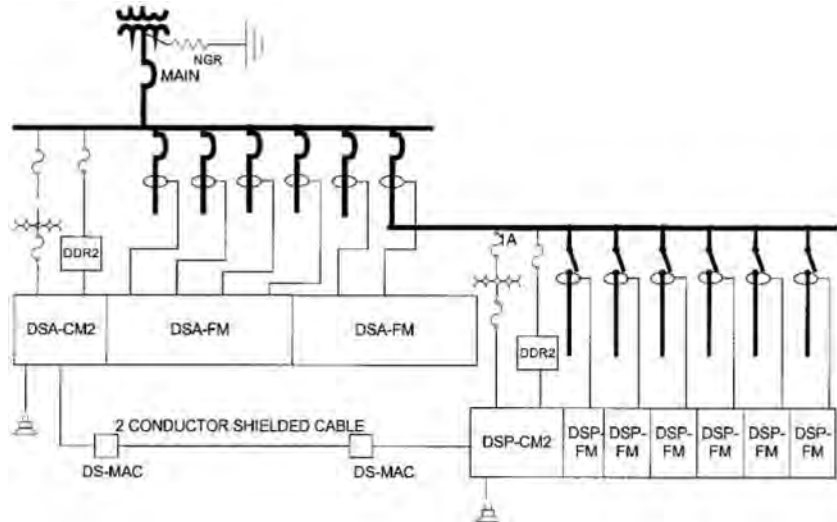
FIGURE 10.3.3 (B): TWO-LEVEL GROUND FAULT SYSTEM WITH DSA ON MAINS AND DSP ON FEEDERS.
