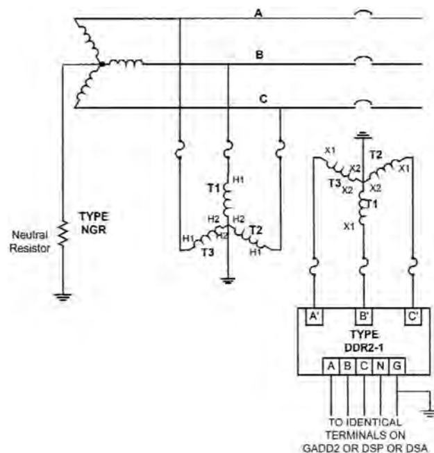
MEDIUM VOLTAGE WYE SYSTEM WITH DDR2-1 CONNECTION.
