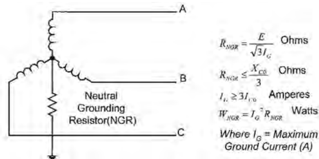
FIGURE 3.1: WYE SYSTEM GROUNDING
