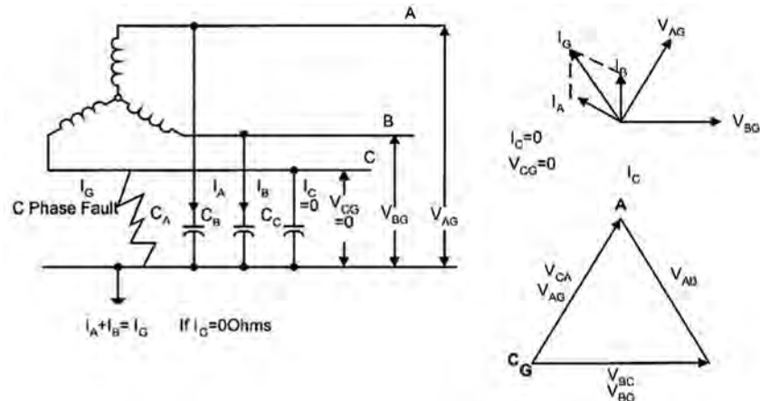
FIGURE 2.1 (B): UNGROUNDED SYSTEM WITH FAULT ON PHASE C
