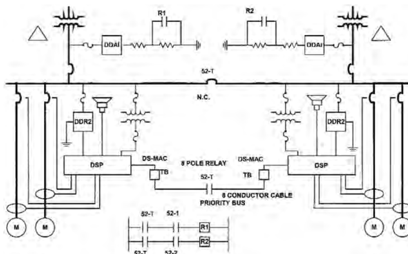
FIGURE 11.6: DOUBLE SOURCE, SINGLE LEVEL DSP PROTECTION WITH NORMALLY CLOSED TIE BREAKER.
