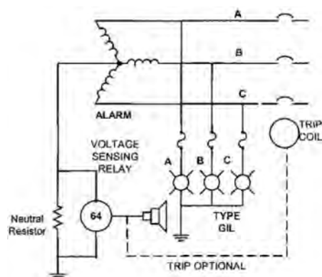
FIGURE 8.1 (B): INDICATION ON WYE SYSTEM WITH CURRENT DERIVED ALARM USING MGFR RELAY.
