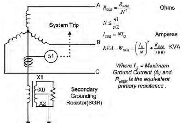
FIGURE 3.2: MEDIUM VOLTAGE WYE SYSTEM GROUNDING
