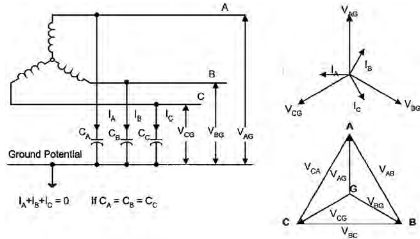
FIGURE 2.1 (A): UNGROUNDED SYSTEM – NORMAL CONDITION
