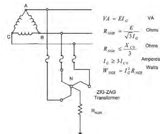
FIGURE 3.3: DELTA SYSTEM GROUNDING
