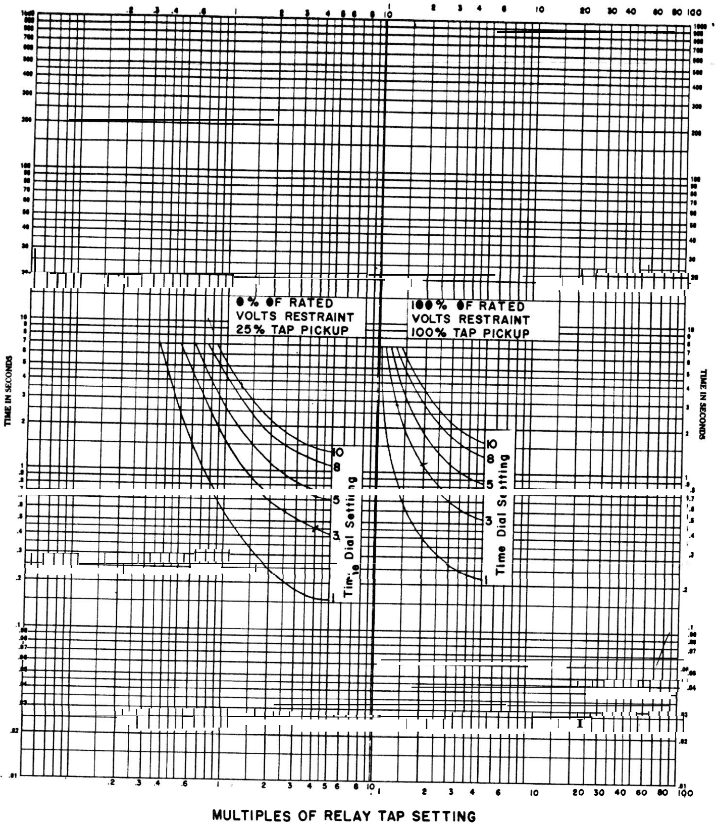
● Ffg. 5 (088880290-0 Sh. 1) Typical Time-current Characteristics of Type IJCV Relay with 0% or 100% of Rated Restraint Voltage.
