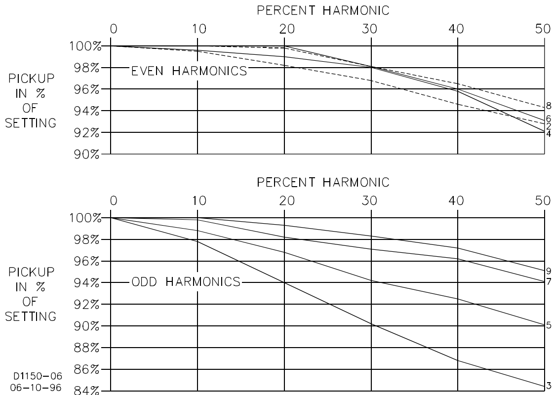
Figure 1-2. Harmonic Rejection
